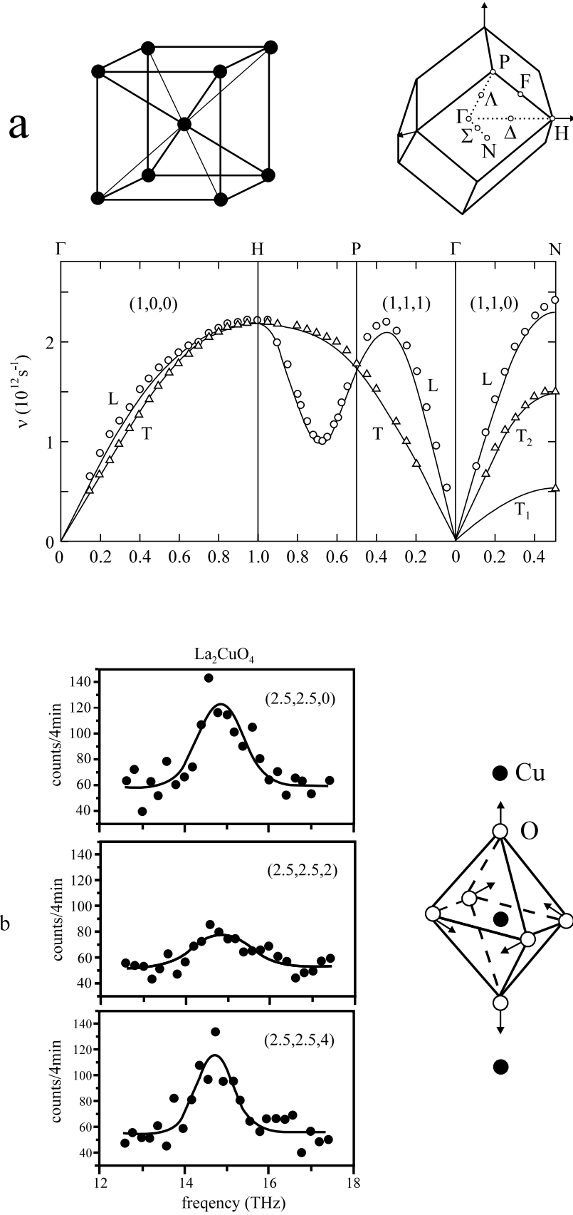
Fig. 7. (a) bcc structure, Brillouin zone, and phonon dispersion curves for potassium. Along the horizontal axis we plot q , q/\sqrt{2} , and q/\sqrt{3} for the (1, 0, 0) , (1, 1, 0) , and (1, 1, 1) directions, respectively. (b) excitation of a particular optical phonon (“scissor” mode) of \text{La}_2\text{CuO}_4 when excited with the participation of different reciprocal lattice vectors. According to Cowley et al.[9] and Pintschovius [10].
